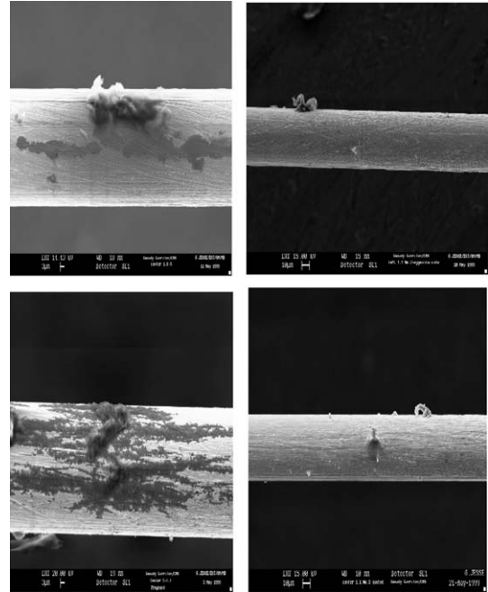
Fig. 11. Anode wires after irradiation as seen with the help of an electron-scanning microscope.
