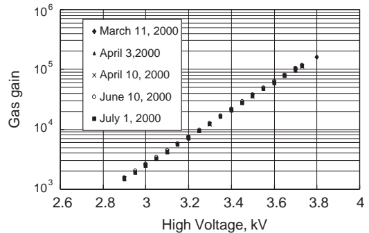
Fig. 5. Gas gain as a function of high voltage at different dates during 6 months of irradiation.
