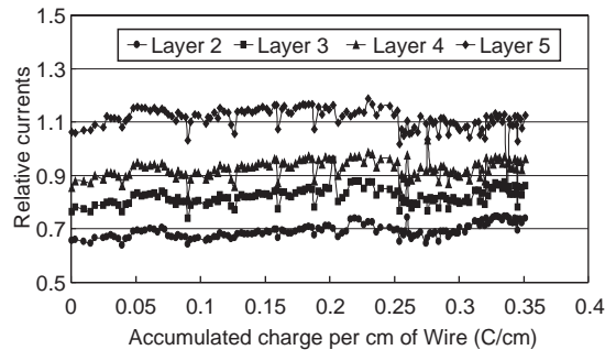
Fig. 6. Relative currents normalized to the average of the 1st and 6th non-irradiated planes, [I_1 + I_6]/2 , vs. accumulated charge.
