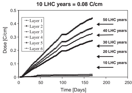
Fig. 3. Accumulation of charge per cm of wire during the half-year test period. Collected charge of 0.08 C/cm is equivalent to 10 LHC years run time. The two outermost layers (1 and 6) were used as reference layers (they had no HV during radiation runs).
