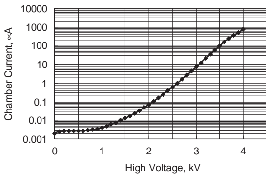
Fig. 4. Chamber current from cathode strips vs. high voltage.
