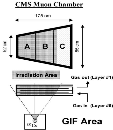
Fig. 2. Schematic diagram of the experimental setup for the aging tests. Two thirds of a chamber were irradiated using the 740 GBq ^{137}\text{Cs} source of the Gamma Irradiation Facility at CERN.
