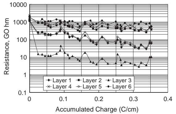
Fig. 9. Resistance between cathode strips vs. accumulated charge.
