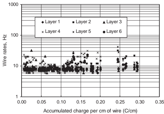
Fig. 7. The variation of the average wire noise count per wire group ( 120\text{ cm}^2 ) vs. accumulated charge.
