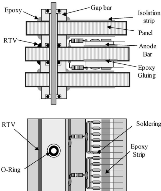
Fig. 1. CMS cathode strip chamber design.
